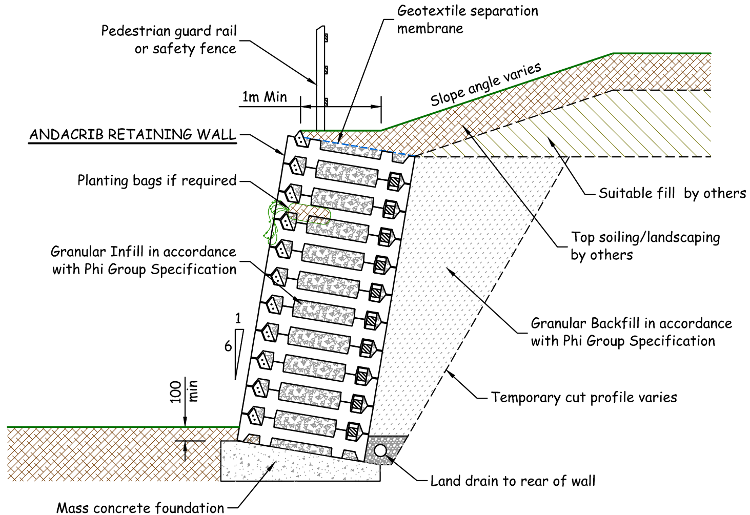
GENERIC SECTION OF ANDACRIB RETAINING WALL
