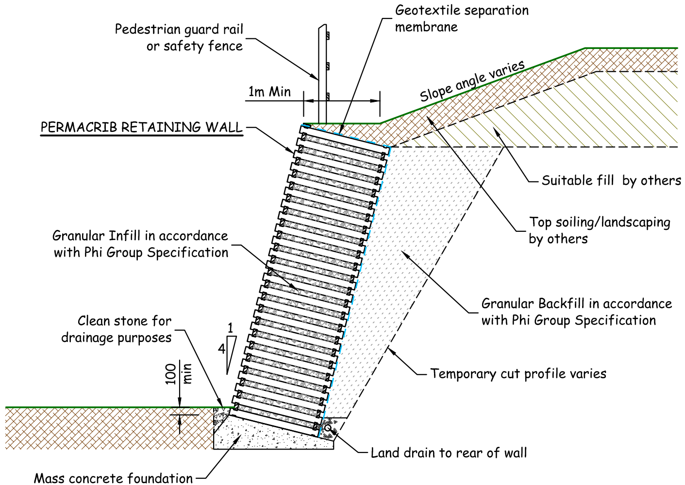
GENERIC SECTION OF PERMACRIB RETAINING WALL
